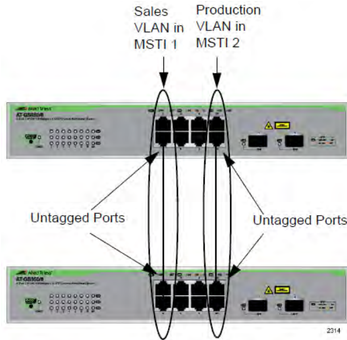
Figure 155. MSTP Example of Two Spanning Tree Instances
