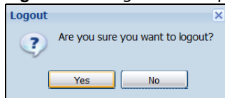
Figure 412 Logout: Prompt
