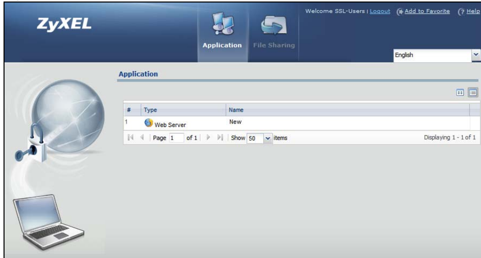
Figure 413 Application
