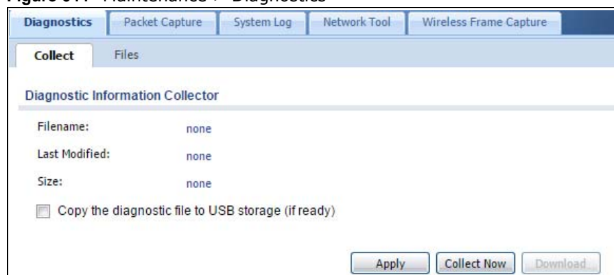
Figure 644 Maintenance > Diagnostics
