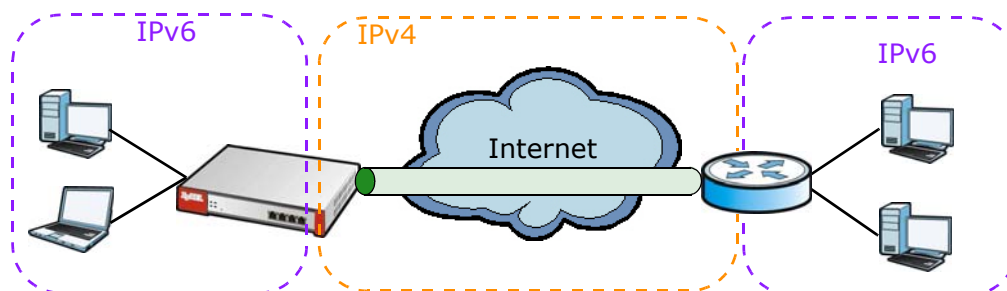
Figure 229 IPv6-in-IPv4 Tunnel
