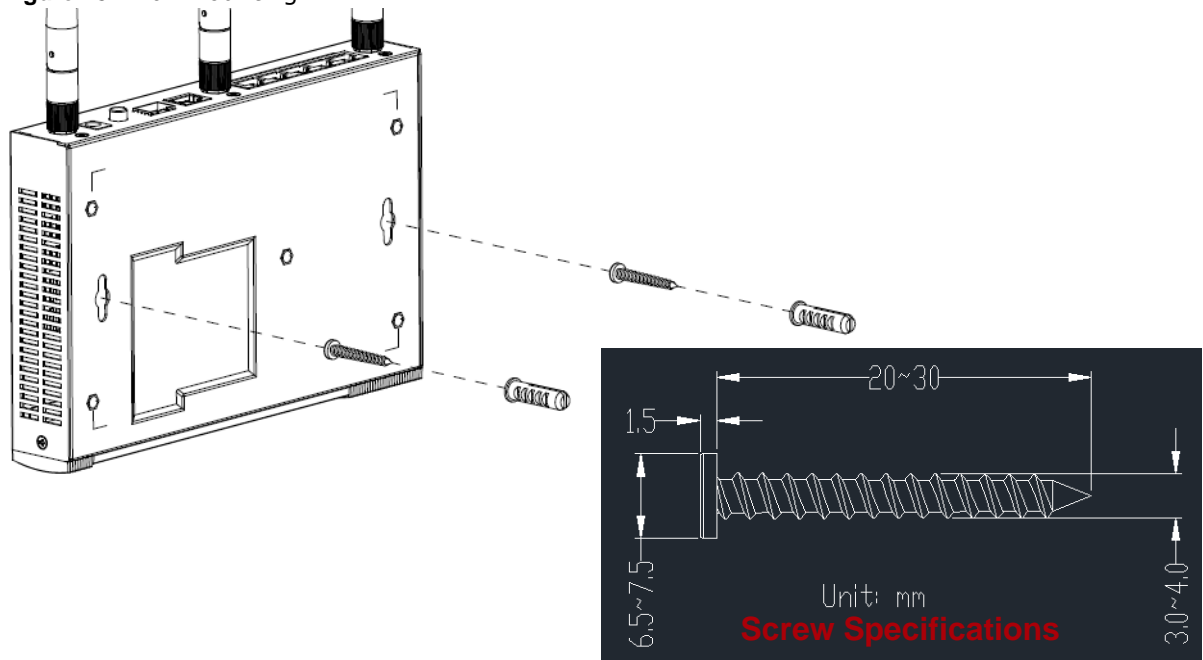
Figure 48 Wall Mounting
