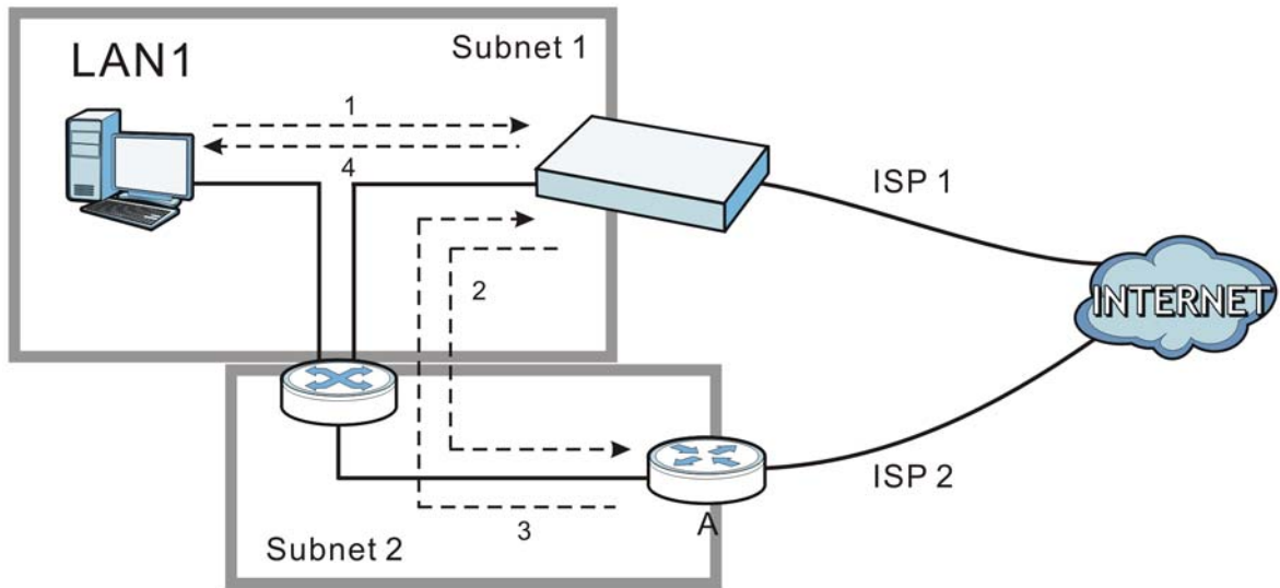
Figure 361 Using Virtual Interfaces to Avoid Asymmetrical Routes
