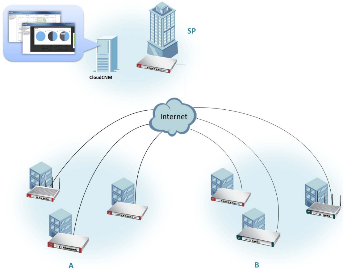
Figure 617 CloudCNM Example Network Topology
