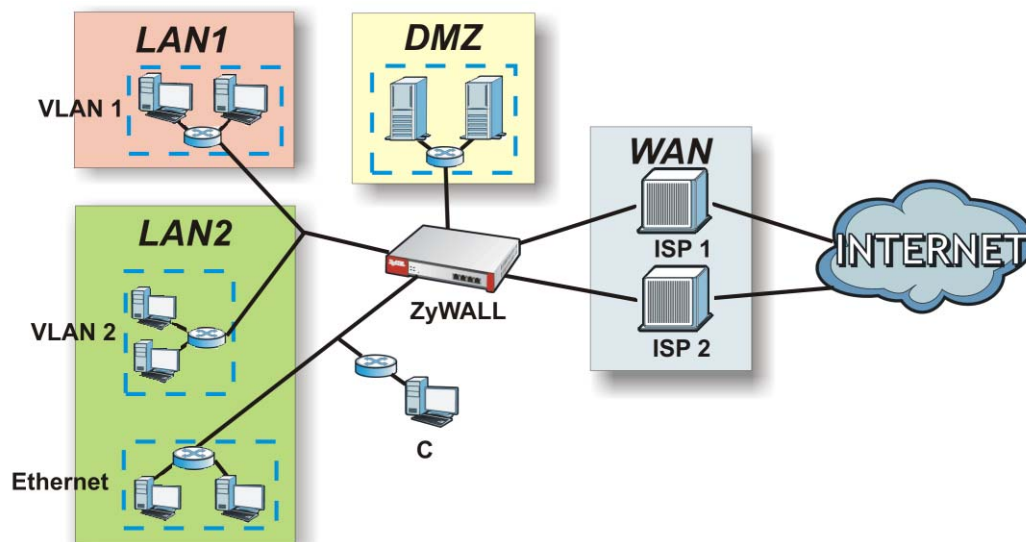
Figure 492 Example: Zones
