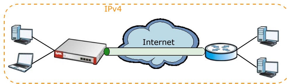
Figure 227 GRE Tunnel Example
