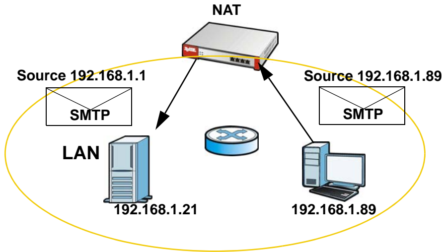
Figure 272 LAN to LAN Traffic
