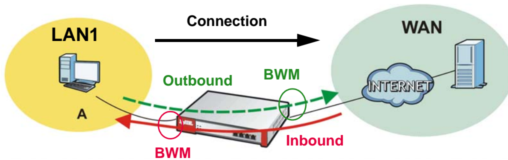
Figure 430 LAN1 to WAN Connection and Packet Directions
