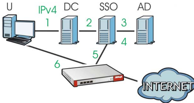
Figure 324 SSO Overview
