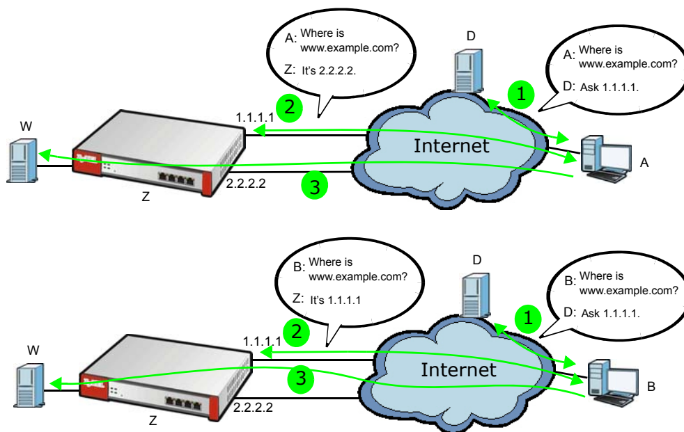
Figure 302 DNS Load Balancing Example
