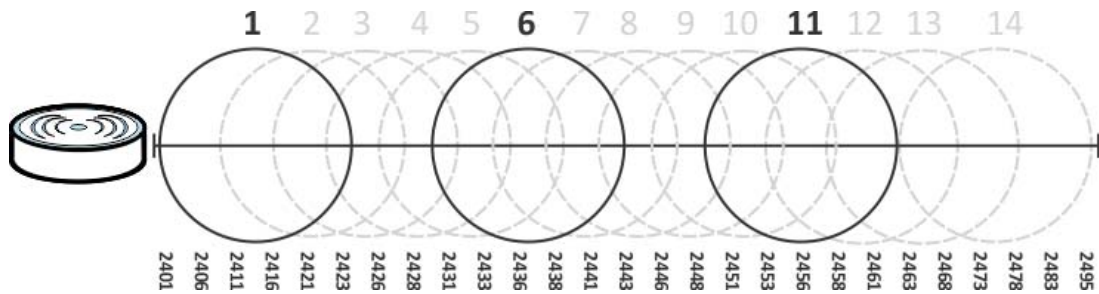
Figure 210 An Example Three-Channel Deployment
