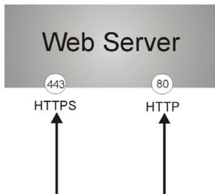
Figure 582 HTTP/HTTPS Implementation
