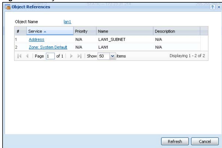
Figure 219 Object References
