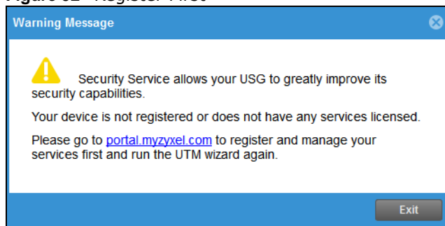
Figure 92 Register First
