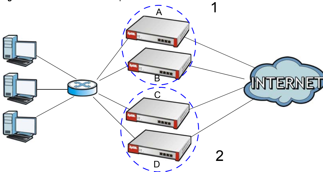
Figure 487 Cluster IDs for Multiple Virtual Routers
