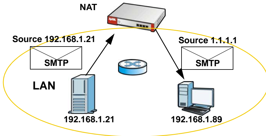
Figure 273 LAN to LAN Return Traffic
