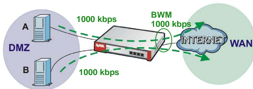
Figure 432 Bandwidth Management Behavior
