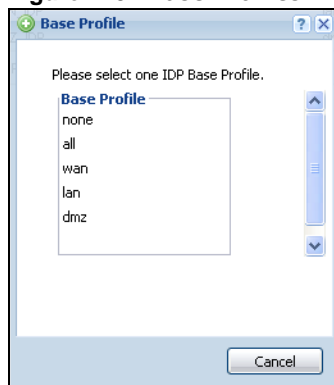
Figure 449 Base Profiles
