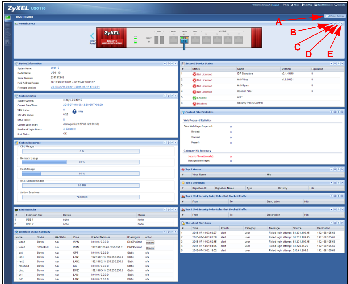
Figure 135 Dashboard
