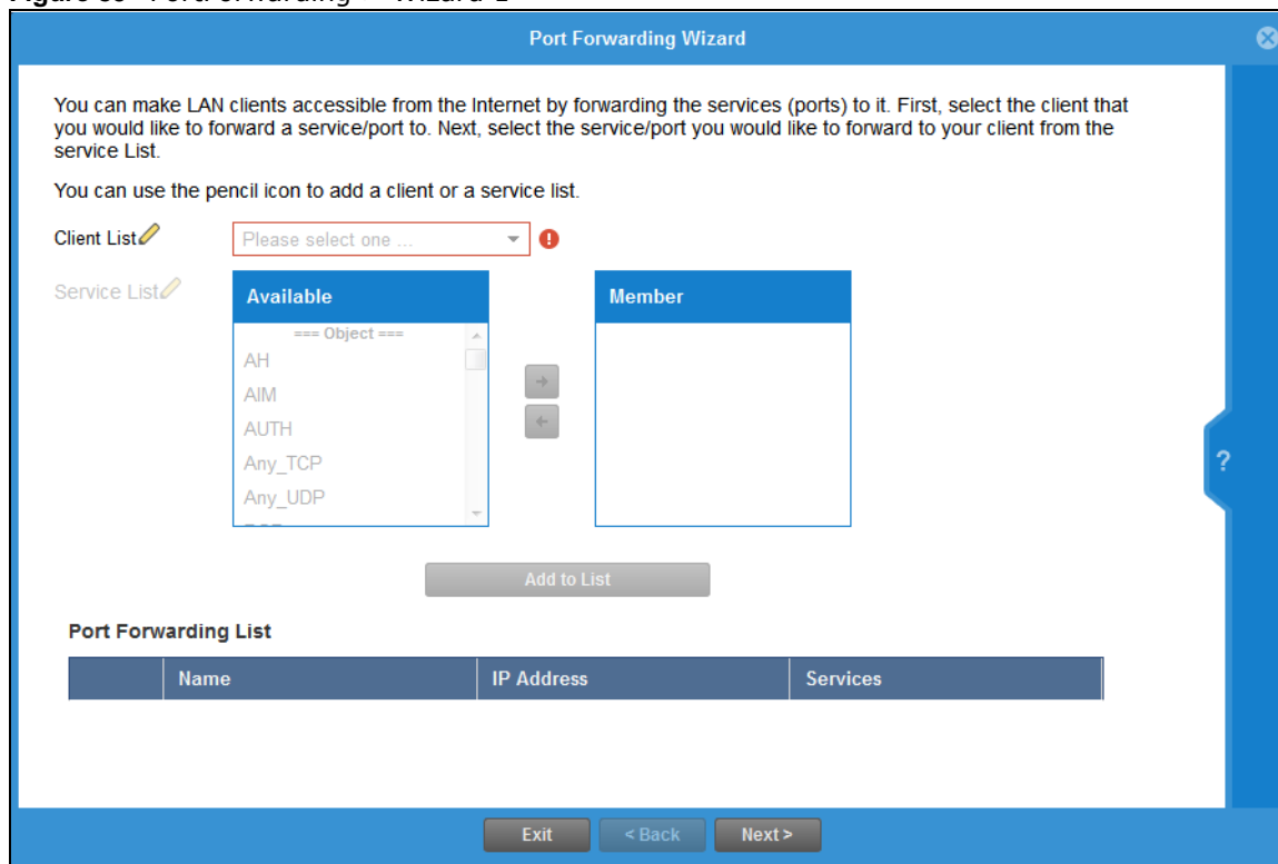
Figure 89 PortForwarding > Wizard 1
