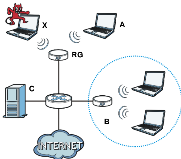
Figure 516 Rogue AP Example
