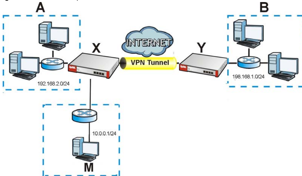
Figure 389 VPN Example: NAT for Inbound and Outbound Traffic
