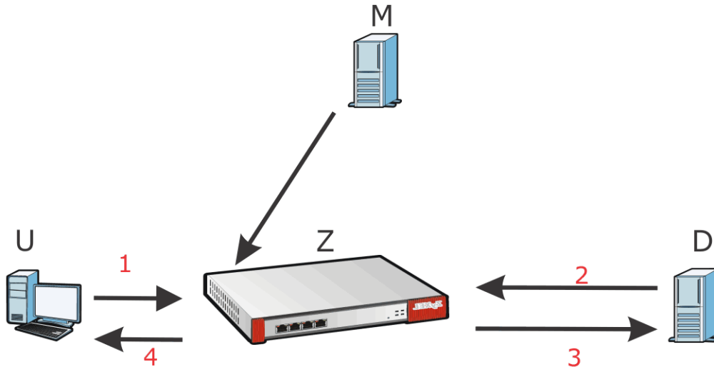
Figure 480 SSL Inspection Certificate Update Overview
