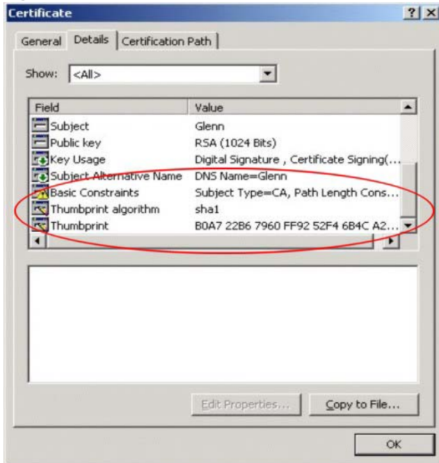
Figure 551 Certificate Details
