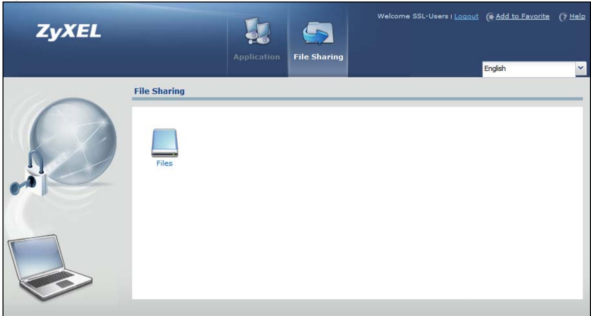
Figure 414 File Sharing
