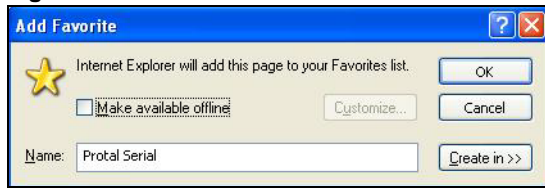
Figure 411 Add Favorite
