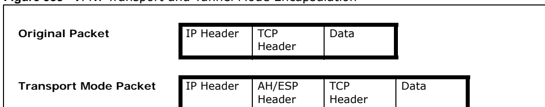
Figure 388 VPN: Transport and Tunnel Mode Encapsulation
