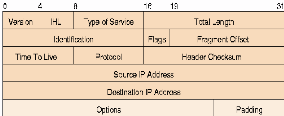
Figure 453 IP v4 Packet Headers
